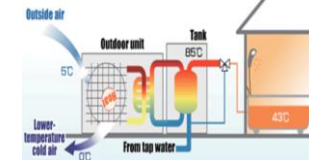
Heat-pump water heater
